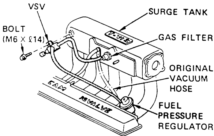
MR2 (P/N 88609-17010) VSV
