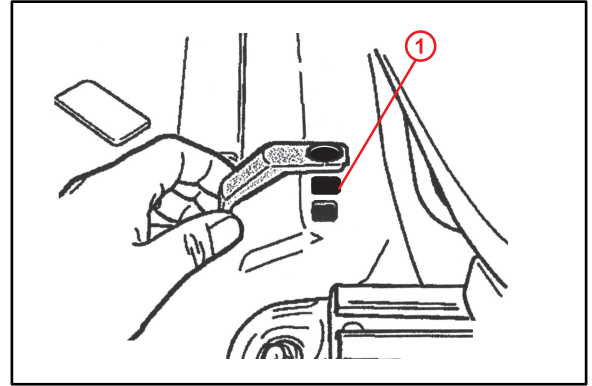
1 Floor Mat Retaining Clip Insert Nut
