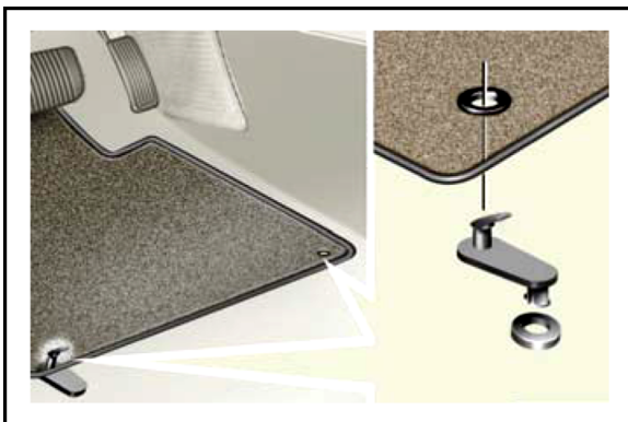
Figure 1. Correct Installation
