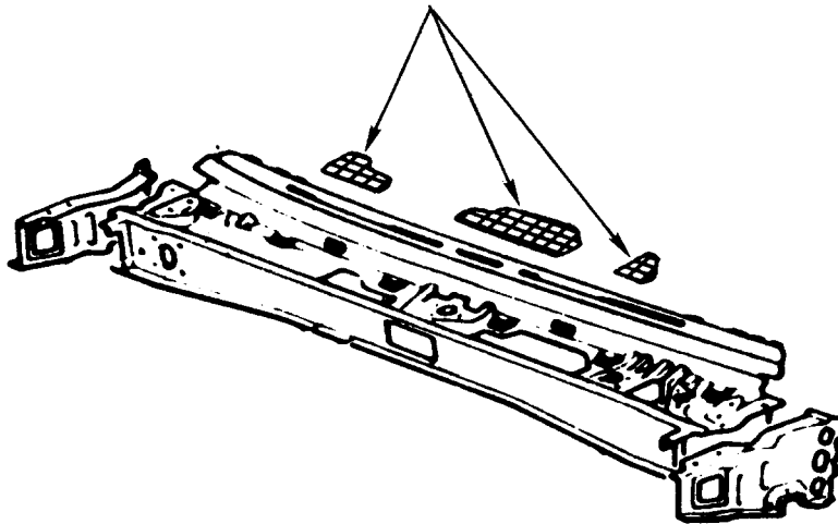
Cowl top ventilator louver (Mesh size: 1.6x1.6mm)
