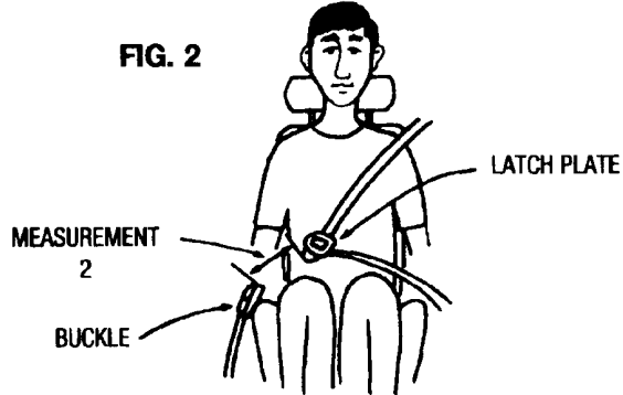
Dimension from latch to buckle
